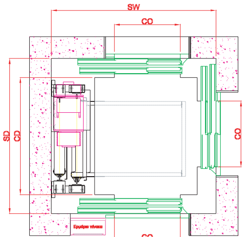
1050 kg / 3 side opening doors
