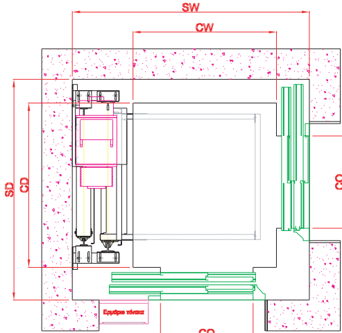
1050 kg / 2 side opening doors
