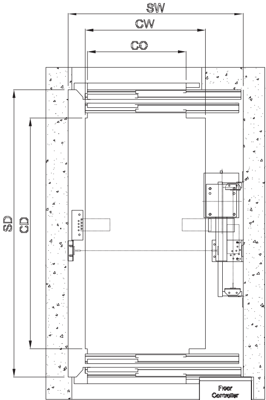
1000 kg / 2 Side Opening Doors
