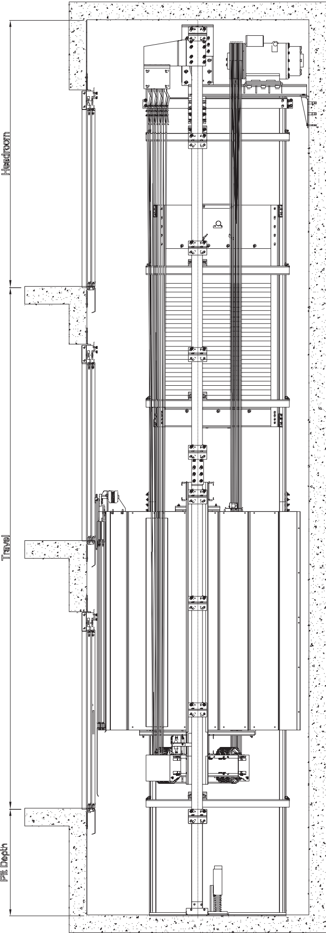
ATLAS MRL GIGAS 2500 Kg
