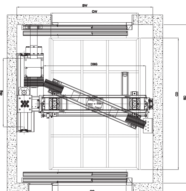
GIGAS 2500 kg / 2 Side Opening Doors
