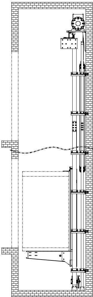
ATLAS MRL 630 Kg
