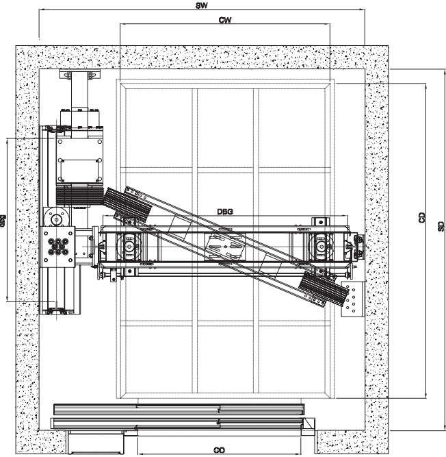
GIGAS 2500 kg / 1 Side Opening Door
